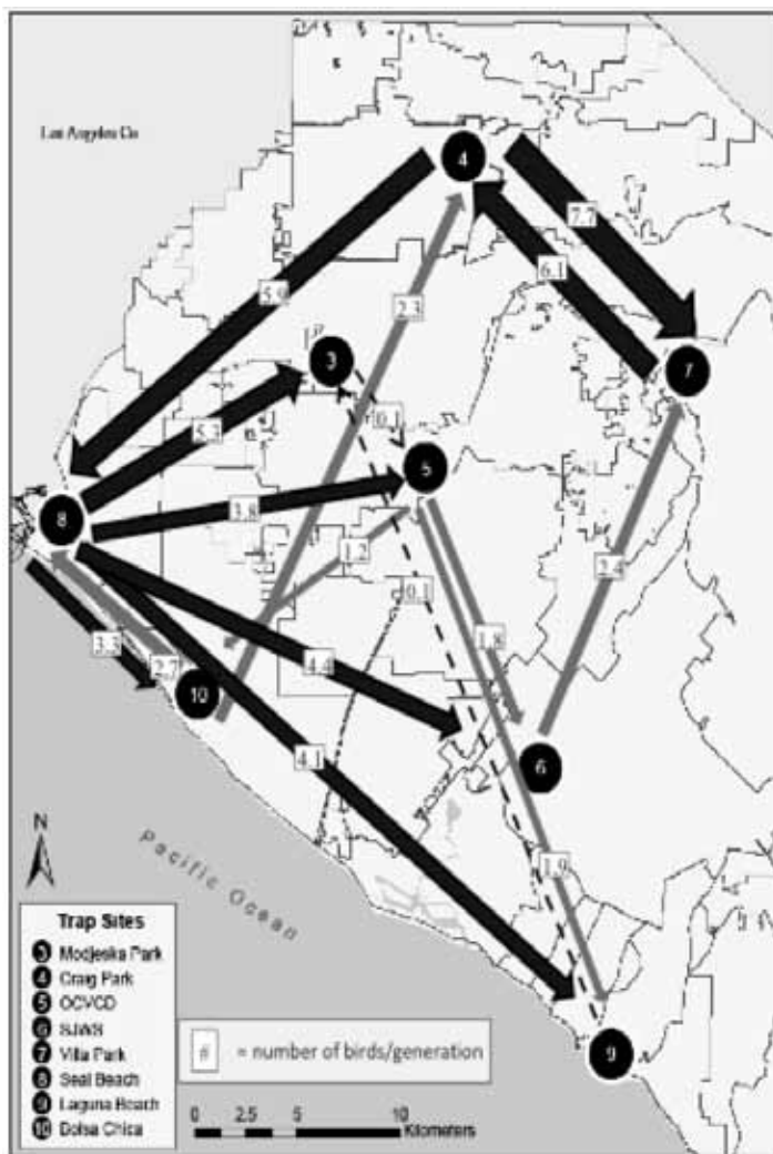
FIGURE 2. Map showing the highest and lowest number of migrants entering each population per generation based on MIGRATE analysis. Arrows represent the magnitude and direction of dispersal and the width of each is proportional to number of migrants (1 migrant = 0.07 cm). Only the highest and lowest dispersal estimates for each population are shown out of the 56 possible pairs for clarity. Dashed arrows indicate < 1 migrant per generation.
