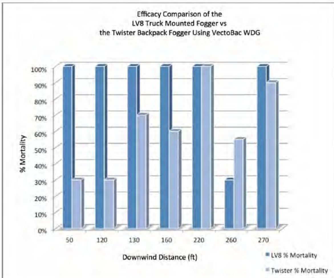
Figure 7. Efficacy comparison of LV8 and Twister sprayers.
