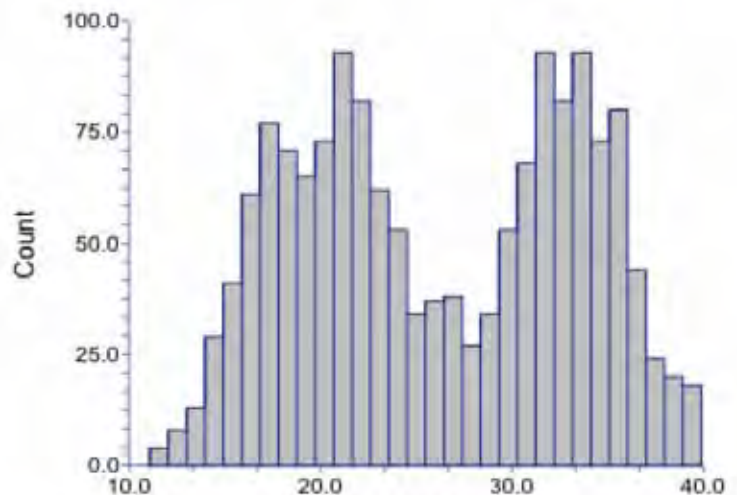
Figure 1. Frequency distribution of Ct scores among dead bird submitted and testing positive for West Nile virus during 2012.
