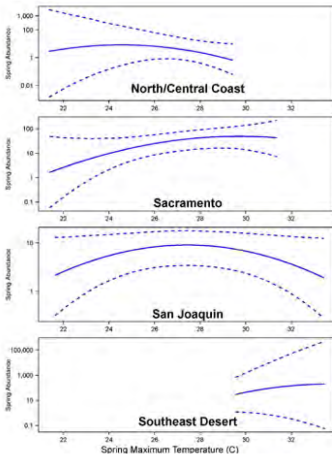
Figure 1. The mean and 95% credibility interval for spring mosquitoes per 30-day trap month from the four significant climate divisions, when predicted by spring maximum temperature.
