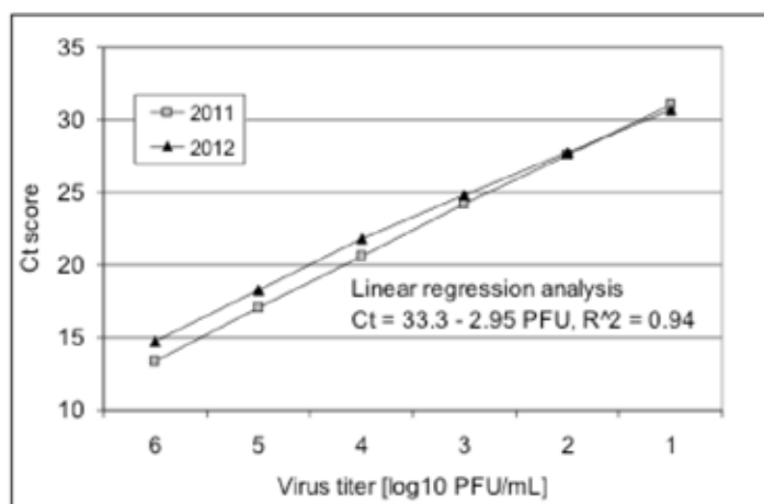
Figure 2. Relationship between Ct score and virus titer determined for samples taken from Vero cell culture and used for proficiency panel testing during 2011 and 2012.
