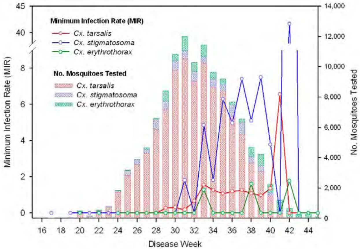
Figure 3. Minimum infection rate and total numbers of mosquitoes tested for WNV from Lake County Large Red Box and CO 2 -baited trap collections graphed by disease week from 2003–2012.
